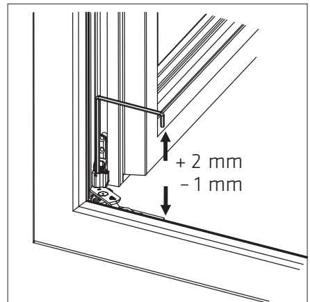
Fig. 1 Height adjustment of sash
