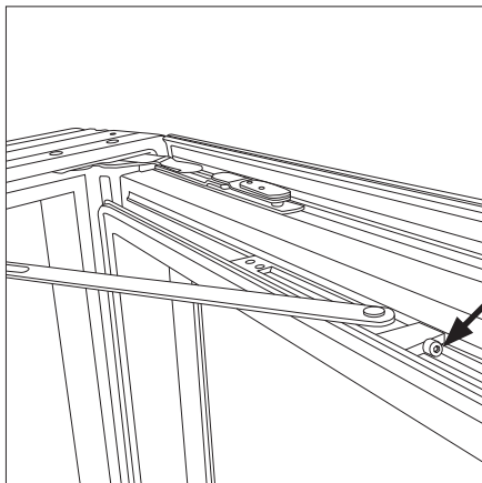
Fig. 6 Adjustment of handle brake
