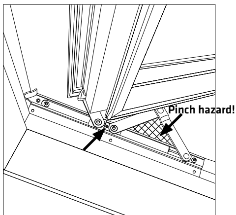
Fig. 4 Adjustment of friction brake
