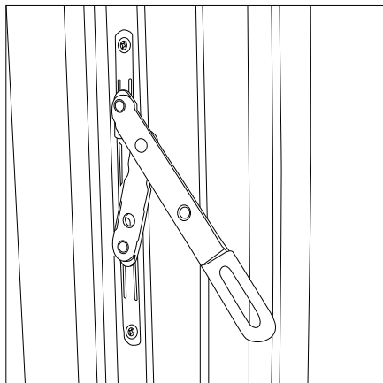
Fig. 7 Concealed handle
